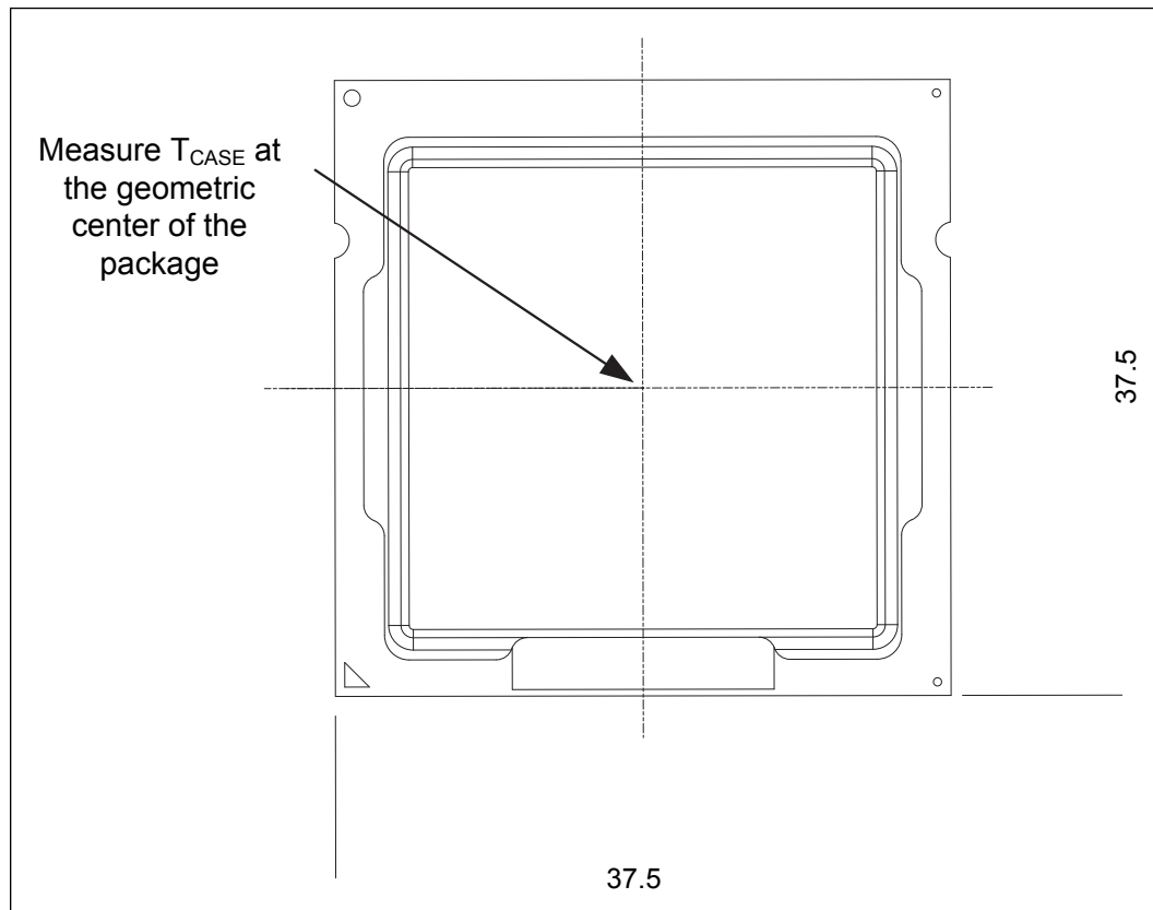
Figure 19. Thermal Test Vehicle (TTV) Case Temperature ( T_{CASE} ) Measurement Location
